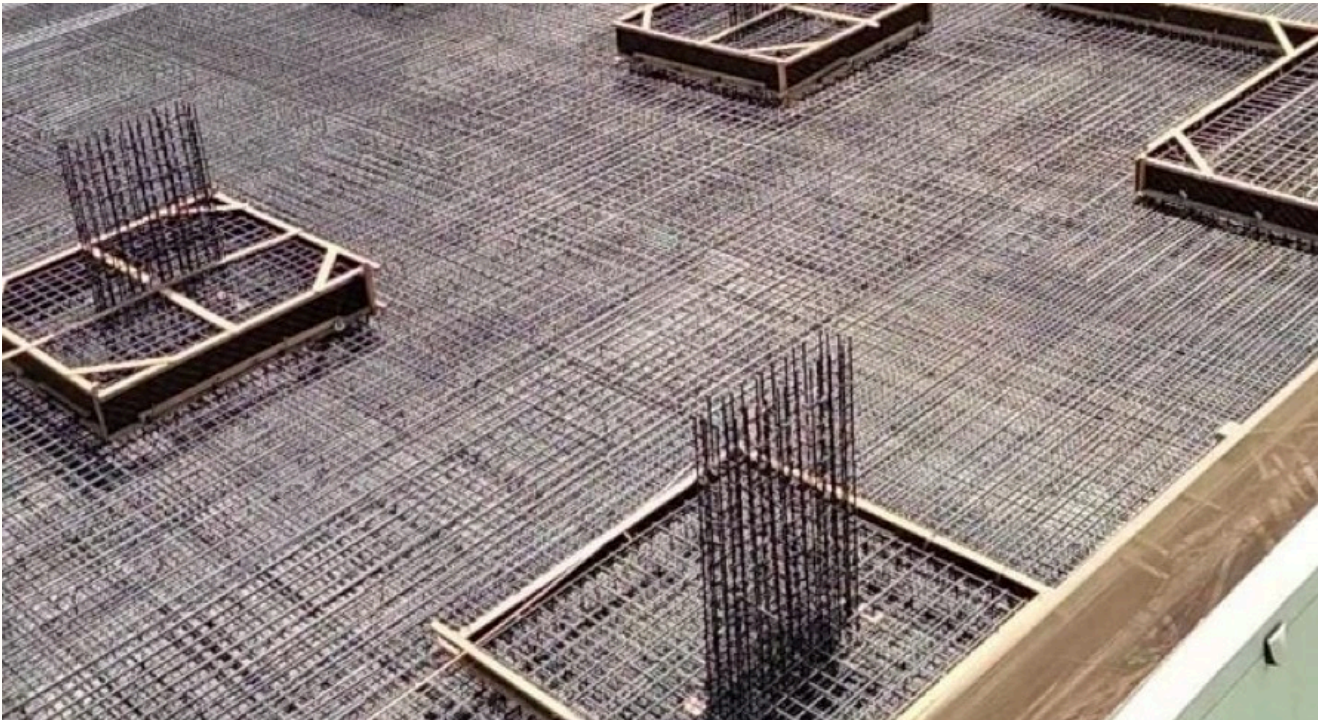
— Raft foundation reinforcement & formwork — column kickers and starter bars
